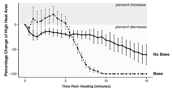
Fig. 6 The average percentage change in the area of the heated region for experimental ( n=434 ) and control ( n=62 ) hives over time. The heated region was defined as the red area above 37^{\circ}\text{C} (see Online Resource 1) for each generated heat map. The percent increase in the experimental hives demonstrates a dramatic increase in the high heat area within the first 5 min; this pattern was not observed in the control hive. The high heat area within the experimental hives—but not the control hive—then rapidly decreased until the high heat region disappeared and the hives were cooled to safe levels ( <37^{\circ}\text{C} ). Data were from seven observation hives and one control hive with comb, two trials were done for each hive. Error bars represent one standard error
